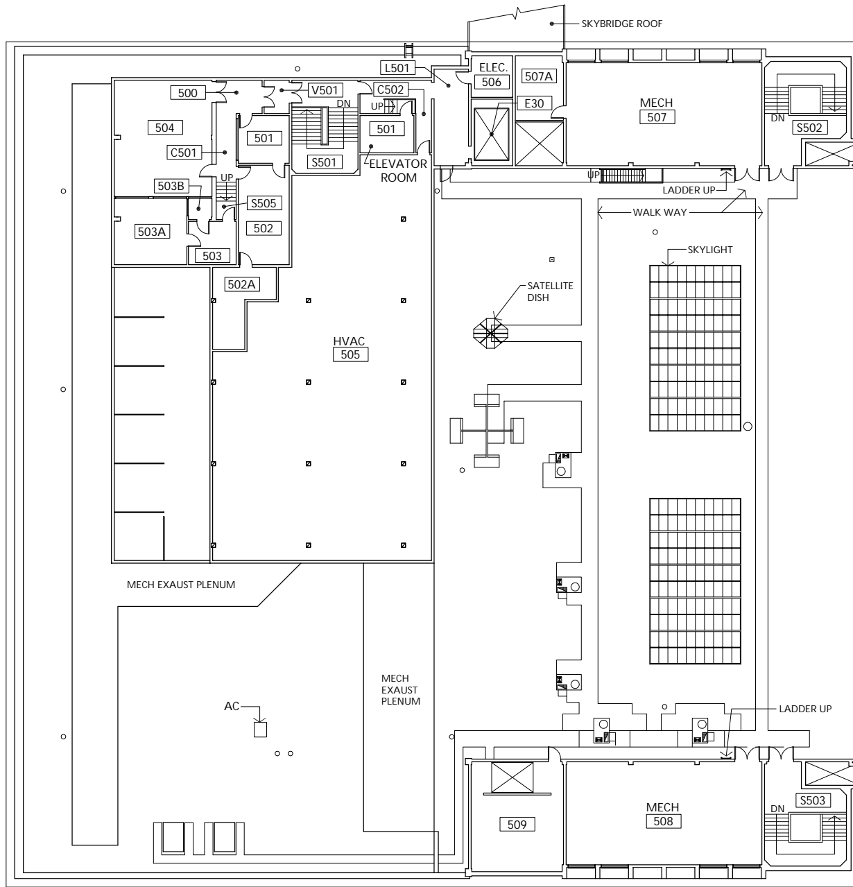
FIFTH FLOOR and PARTIAL ROOF PLAN
