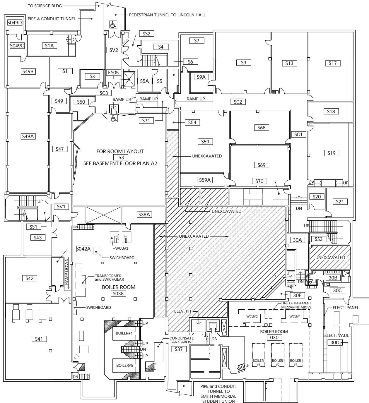
SUB - BASEMENT FLOOR PLAN
